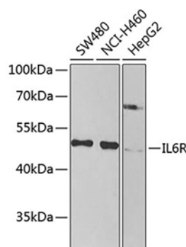
Fig. 1. Western blot analysis of extracts of SW480 cells, using IL6R antibody at 1:1000 dilution. Secondary antibody: HRP-labeled Goat Anti-Rabbit IgG(H+L) (A0208) at 1:1000 dilution. Lysates/proteins: 25μg per lane. Blocking buffer: QuickBlock™ Blocking Buffer (P0231). Detection: BeyoECL Star (P0018A). Exposure time:1s.
